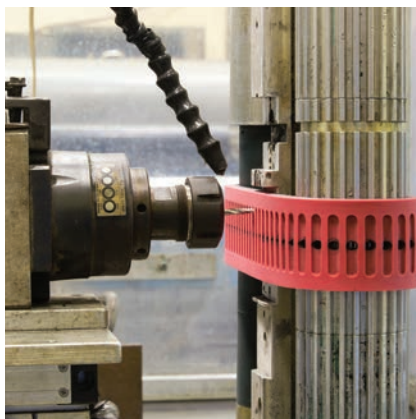
ROUTED SLOT
